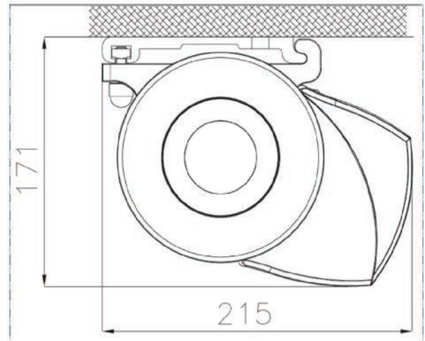
CEILING MOUNTING (mm)
